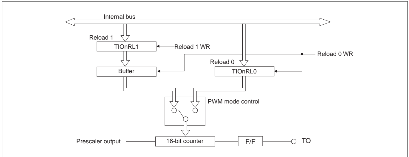
Figure 10.4.10 PWM Circuit Diagram
