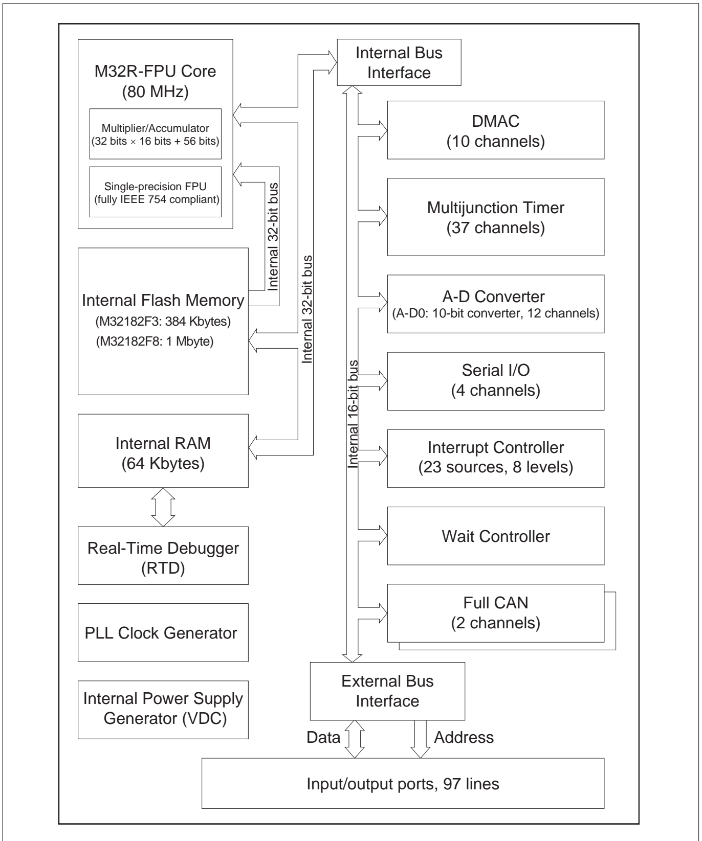
Figure 1.2.1 Block Diagram of the 32182
