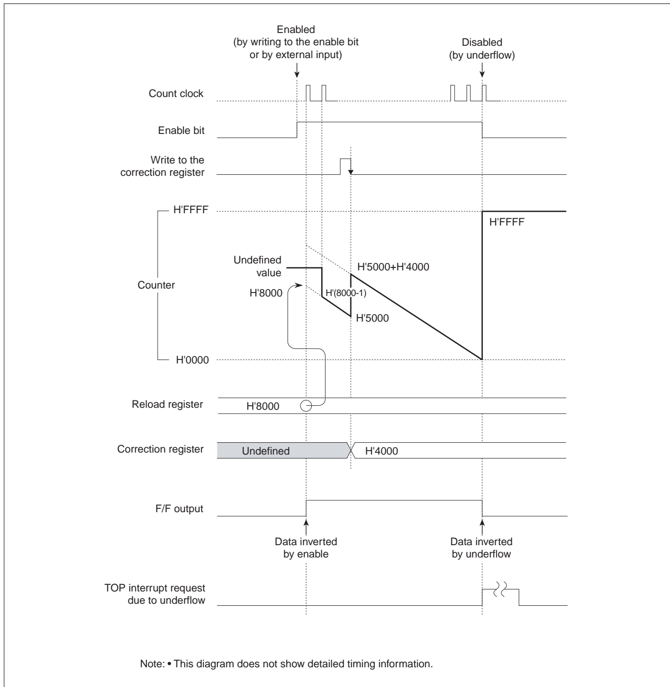
Figure 10.3.10 Typical Operation in TOP Single-shot Output Mode When Count is Corrected
