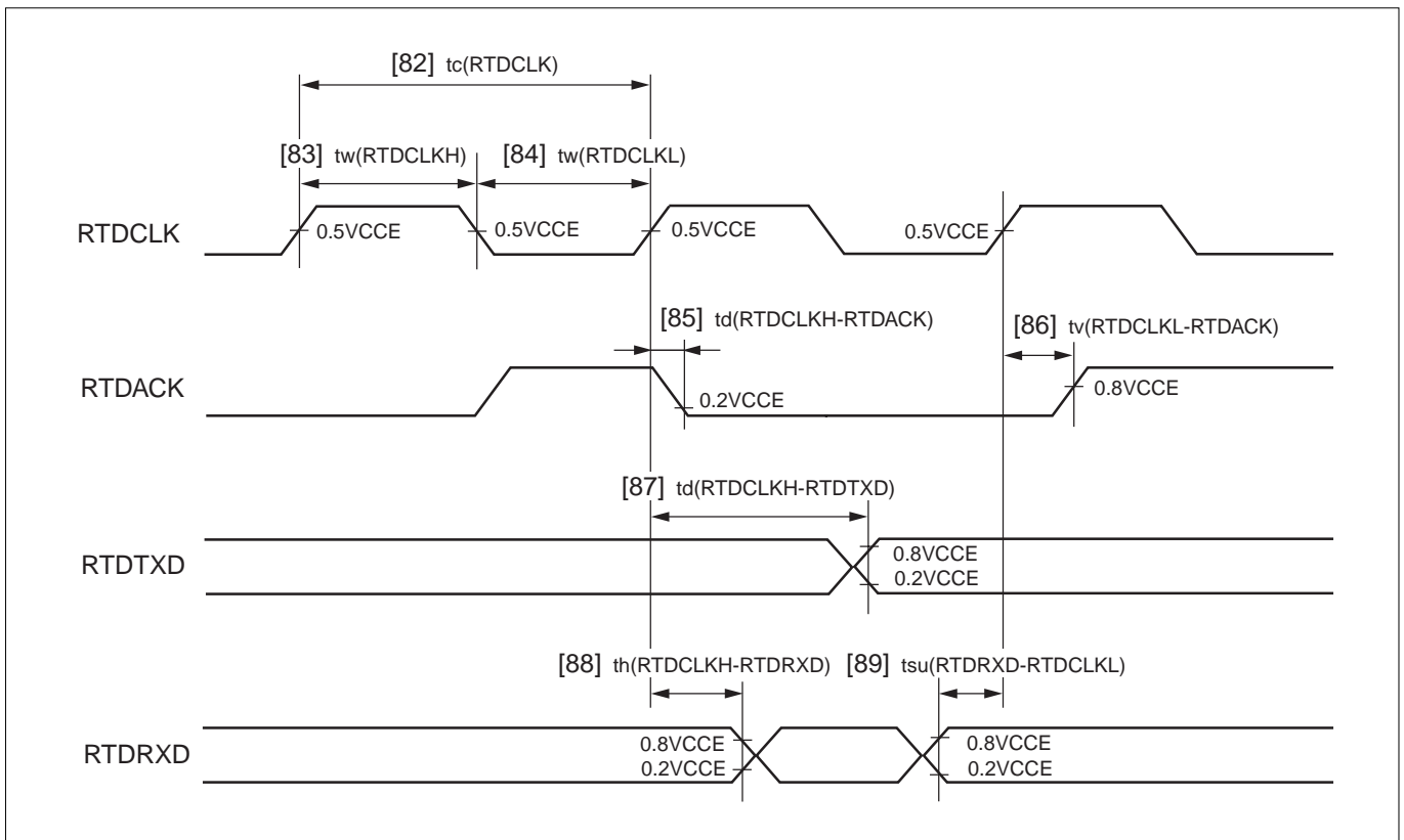
Figure 21.7.14 RTD Timing
