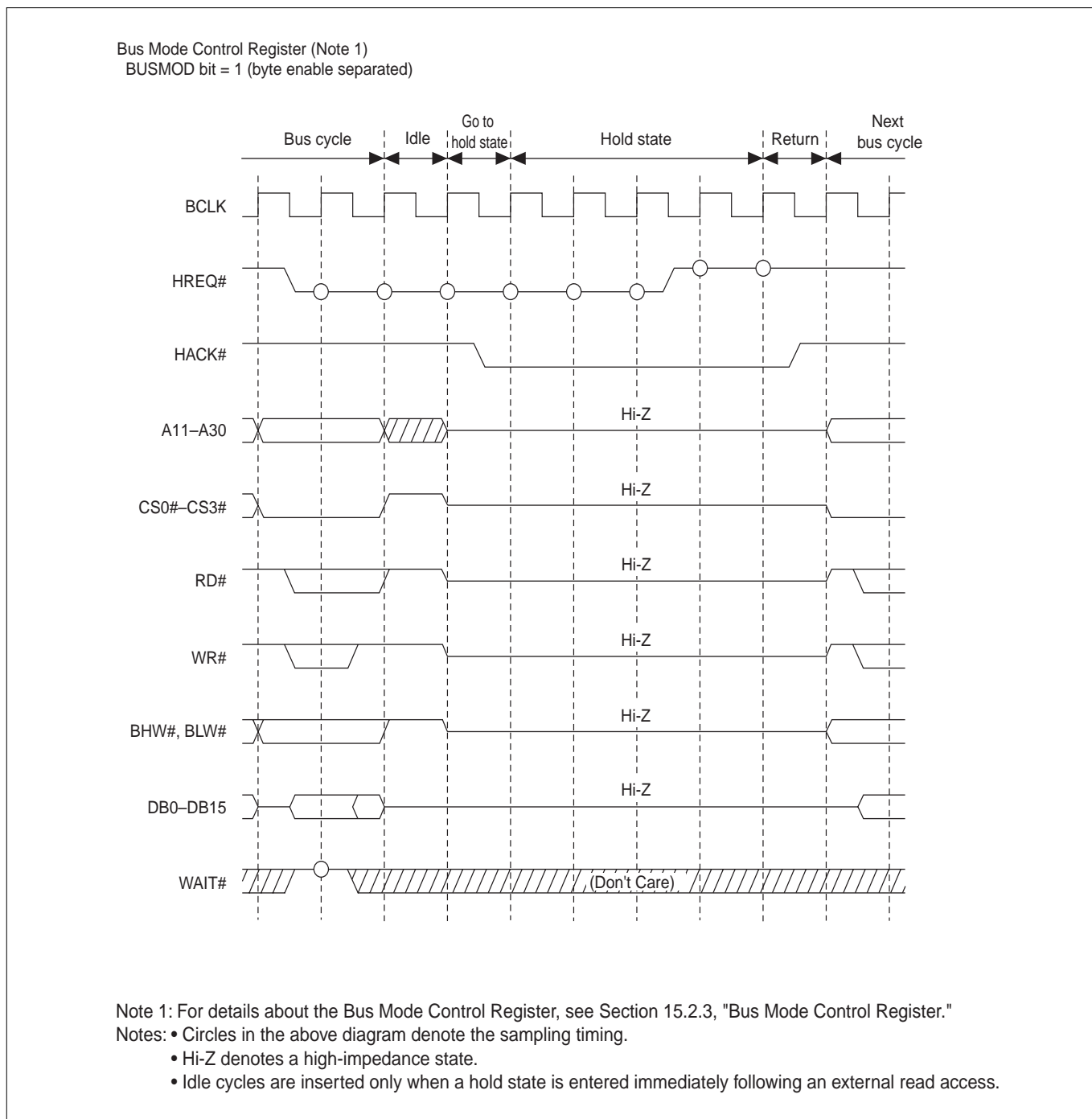
Figure 15.4.2 Bus Arbitration Timing
