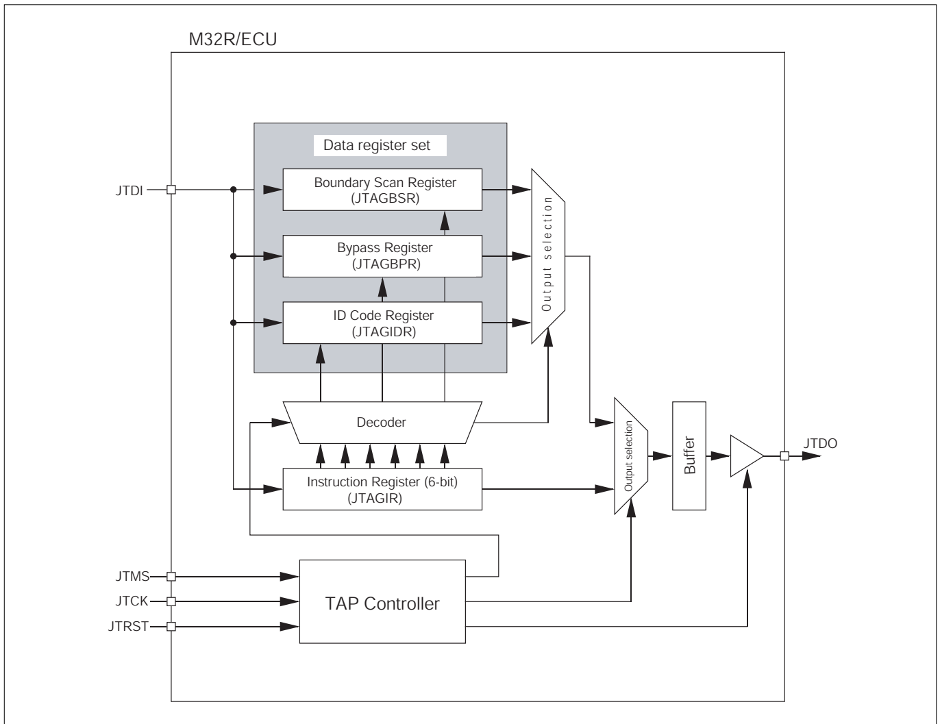
Figure 19.2.1 Configuration of the JTAG Circuit
