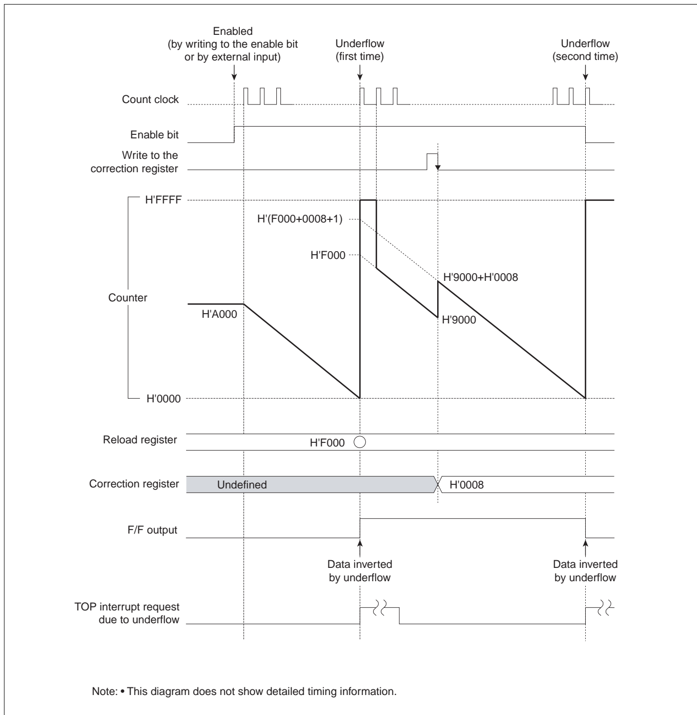
Figure 10.3.15 Typical Operation in TOP Delayed Single-shot Output Mode when Count is Corrected
