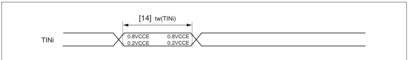
Figure 21.8.5 TINi Timing
