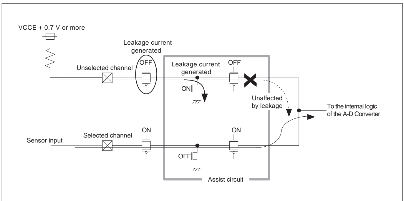
Figure 11.4.2 Example of an Inflow Current Bypass Circuit where VCCE + 0.7 V or More is Applied
