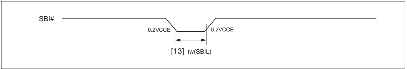
Figure 21.7.3 SBI Timing
