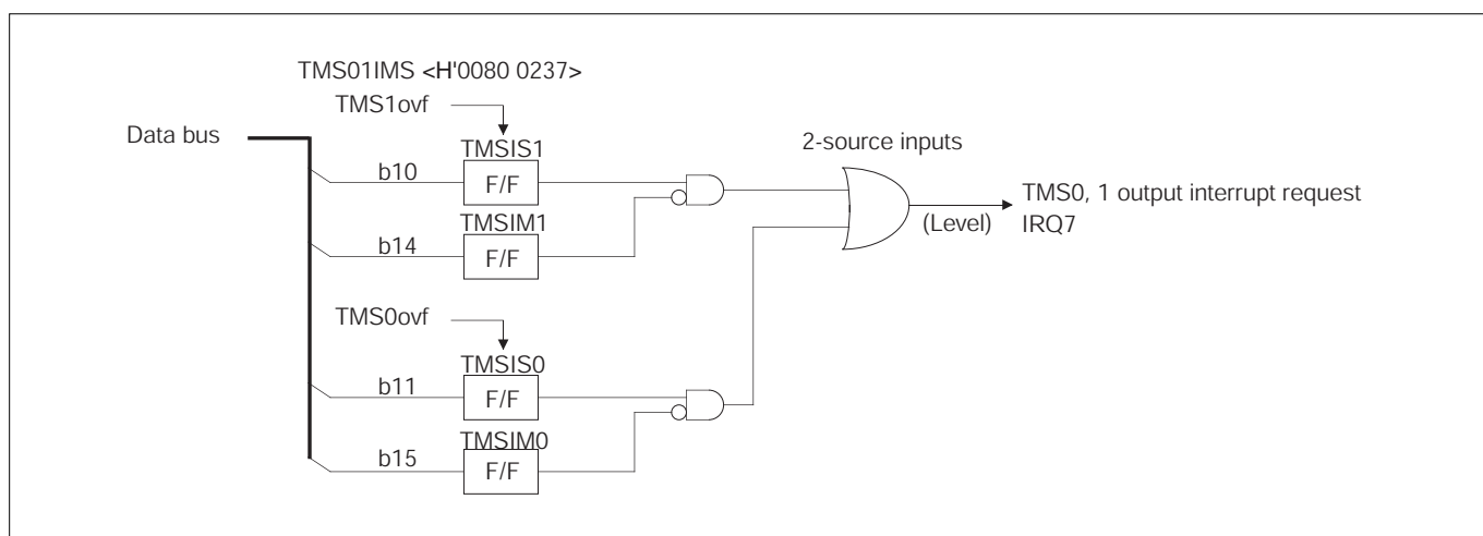
Figure 10.2.11 Block Diagram of TMS0,1 Output Interrupt Request
