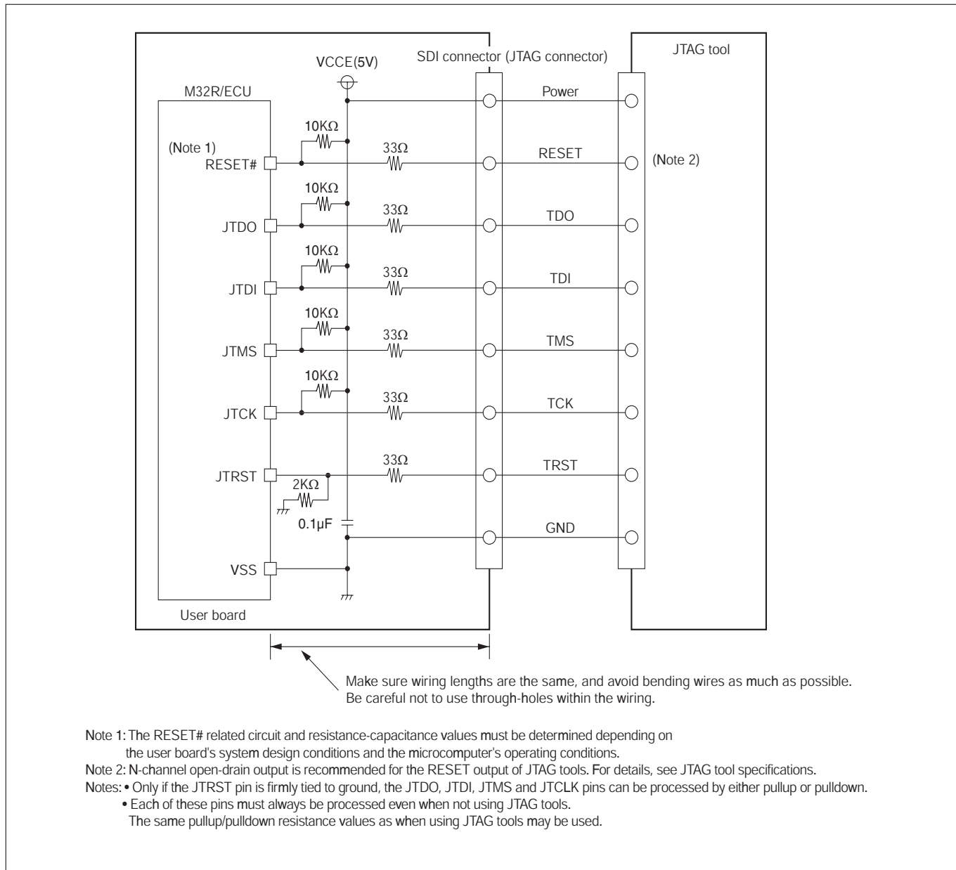
Figure 19.6.1 Notes on Board Design when Connecting JTAG Tools
