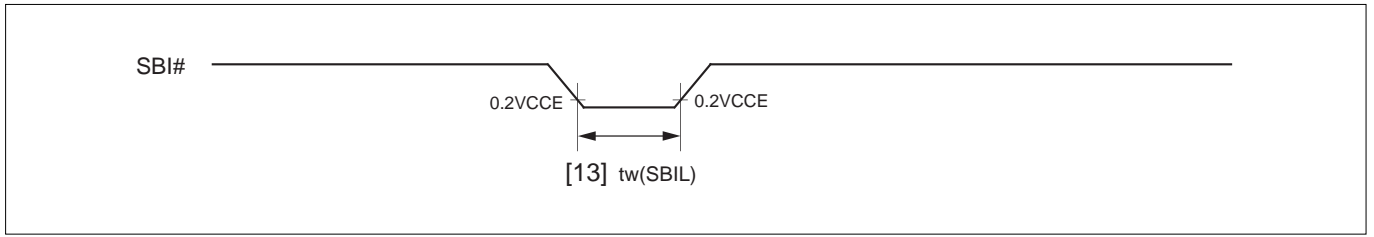
Figure 21.8.3 SBI Timing
