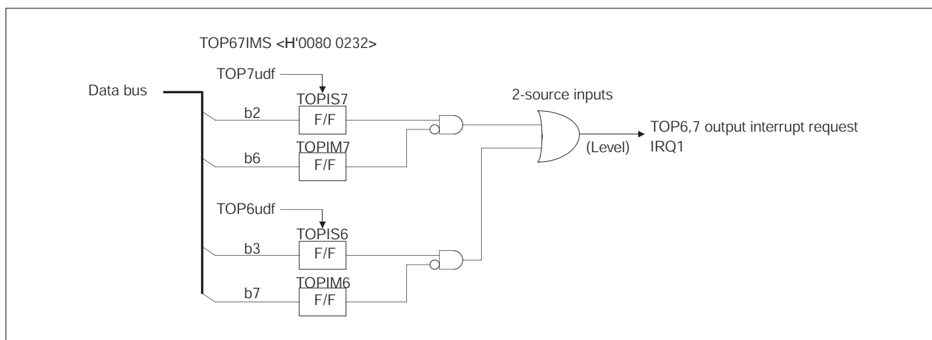
Figure 10.2.6 Block Diagram of TOP6,7 Output Interrupt Request
