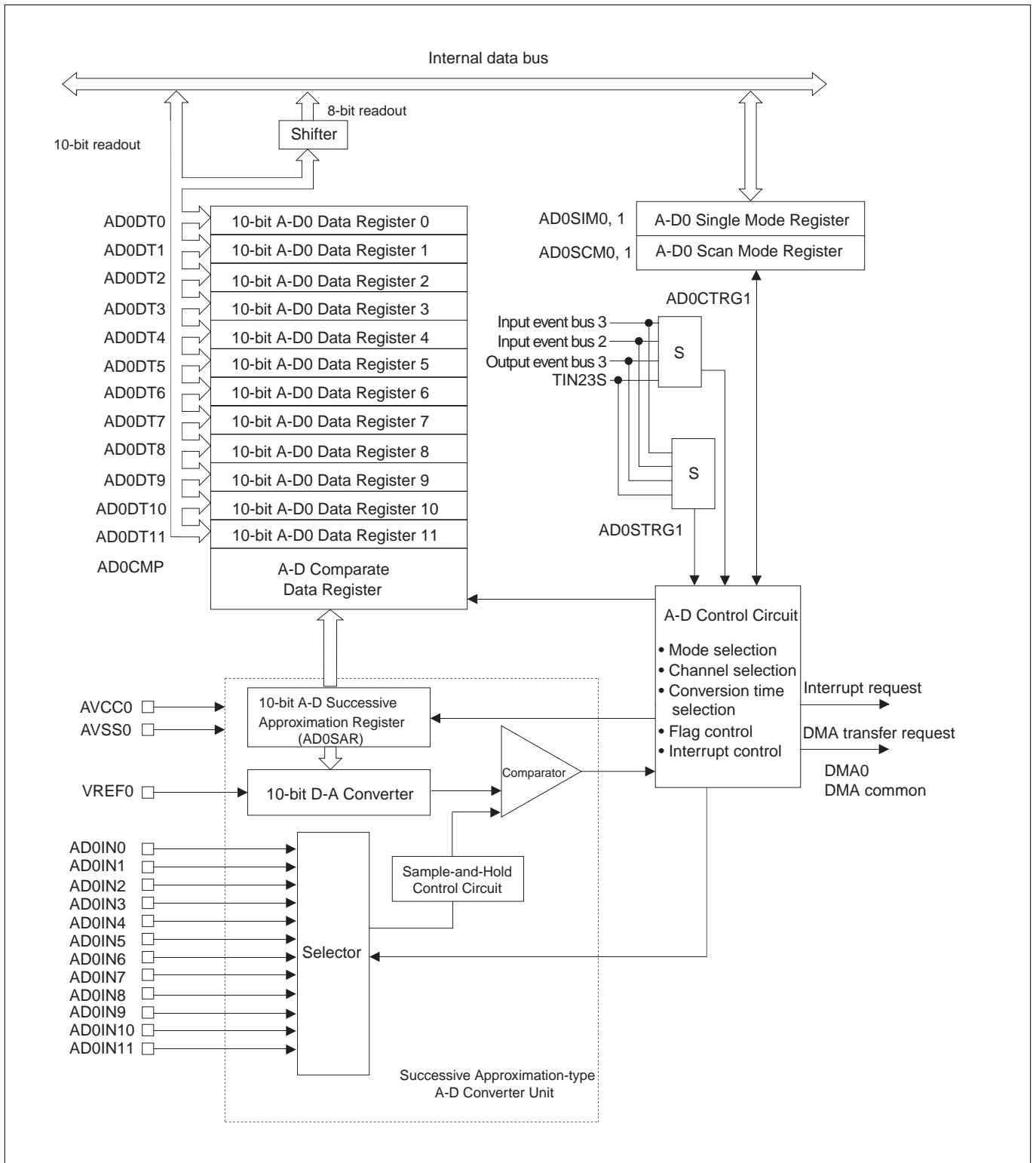
Figure 11.1.1 Block Diagram of the A-D0 Converter
