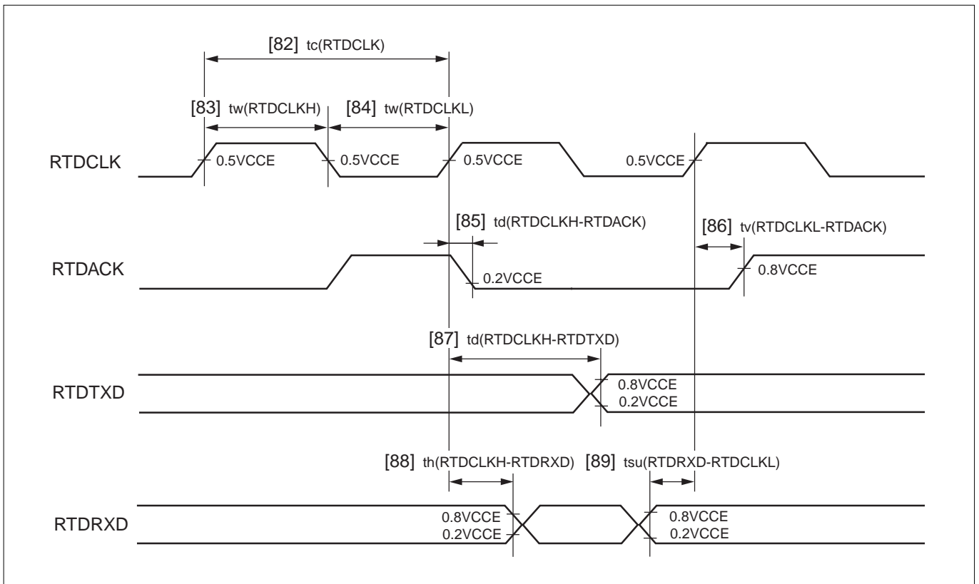
Figure 21.8.14 RTD Timing
