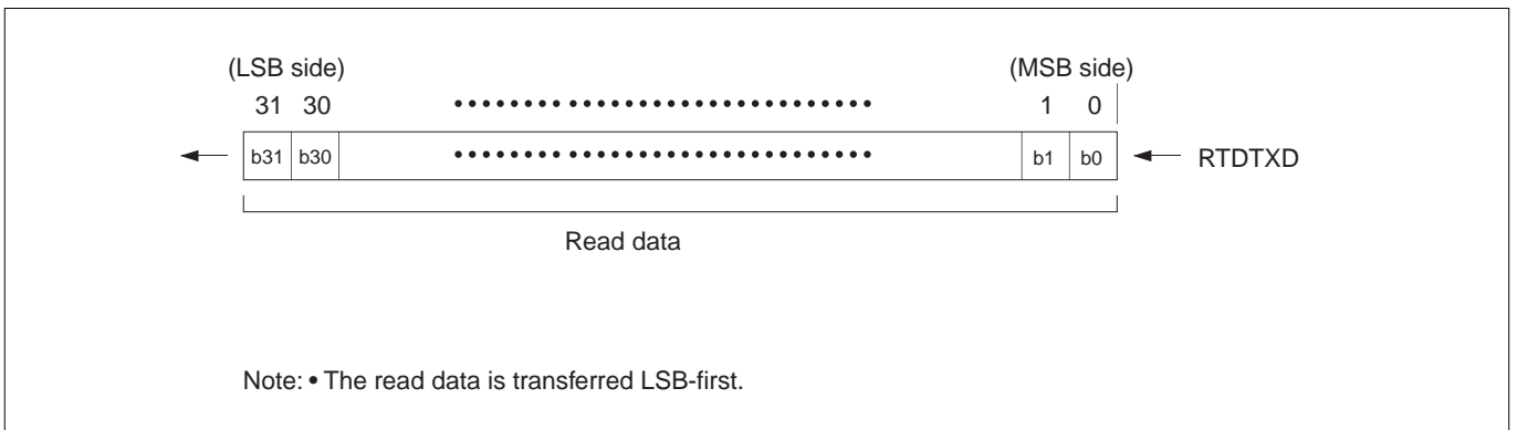
Figure 14.3.3 Read Data Transfer Format
