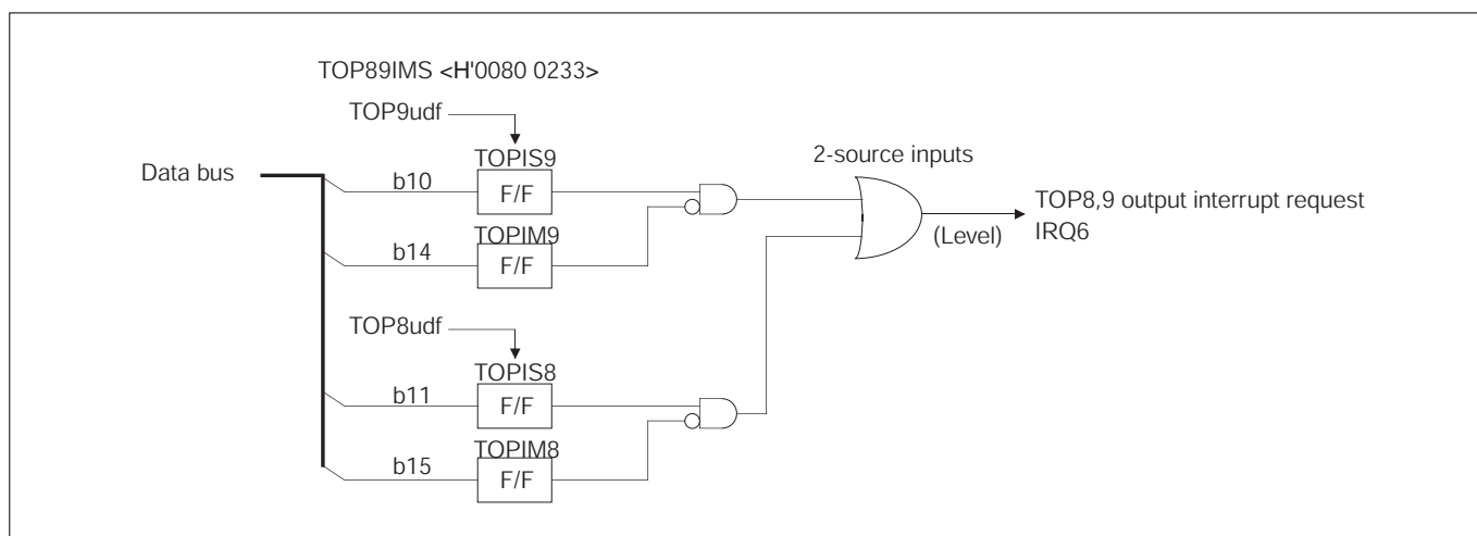
Figure 10.2.7 Block Diagram of TOP8,9 Output Interrupt Request
