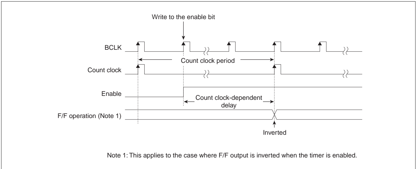
Figure 10.3.2 Count Clock Dependent Delay
