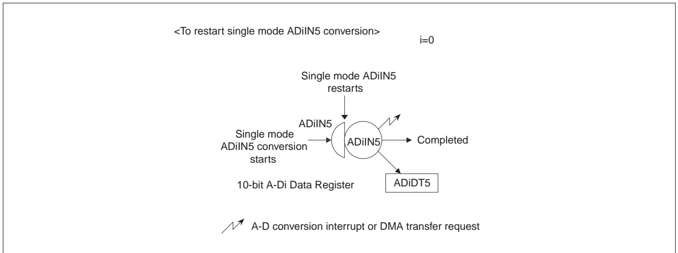
Figure 11.1.7 Conversion Restart during Single Mode Operation
