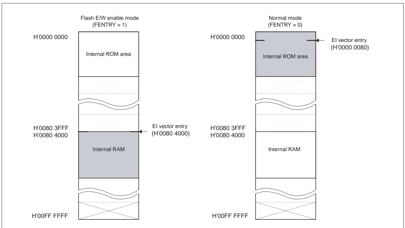
Figure 6.5.1 EI Vector Entry during Flash E/W Enable Mode
